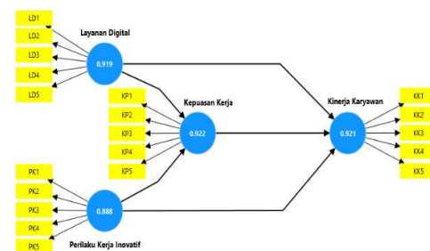
graphic 5. Reliabilitas Komposit
