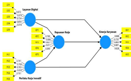
graphic 2. Outer Loading
