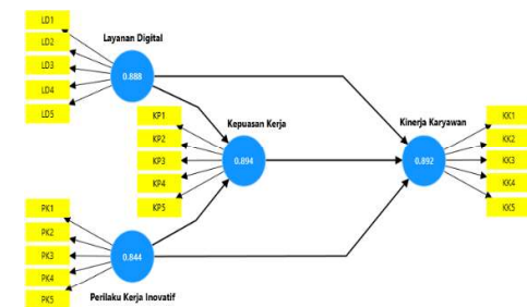
graphic 4 Cronbach' Alpha
