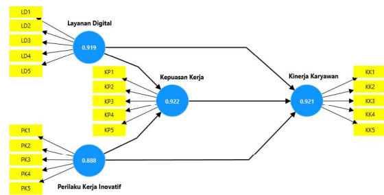
graphic 6. R Square
