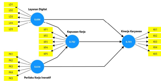
graphic 7 Nilai AVE
